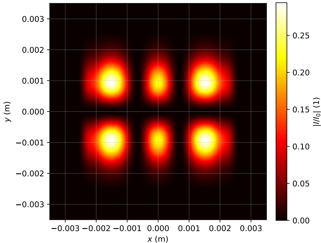
Intensity profile I(x, y, z = 3.264)/I_0 , P_{in}=0.5P_{cr} , artificial time
